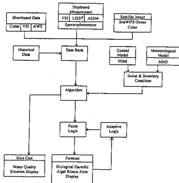
Figure 1 Schematic of the PREPP
